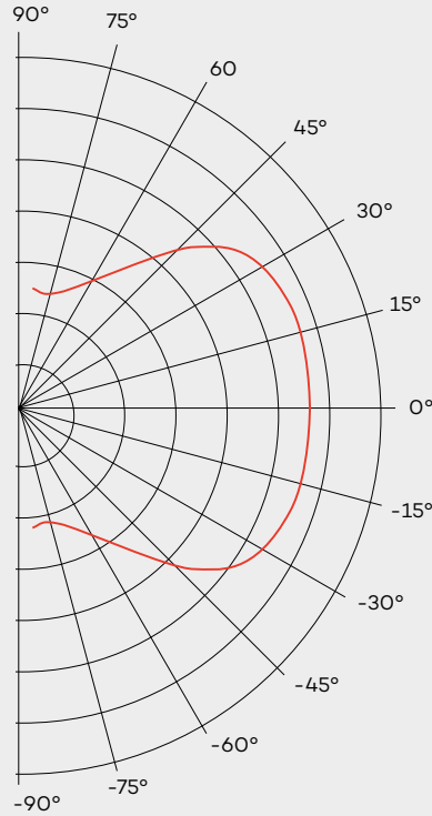
Fig. 2: Glare suppression of PLEXIGLAS® Textures for Luminaires OA000 SL for edge-lit LED ceiling lights
