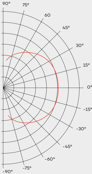
Fig. 1: Performance of a standard light-diffuser panel
