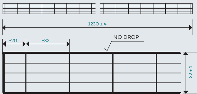
Cross-section of PLEXIGLAS® Resist S5P 32 (dimensions in mm)
