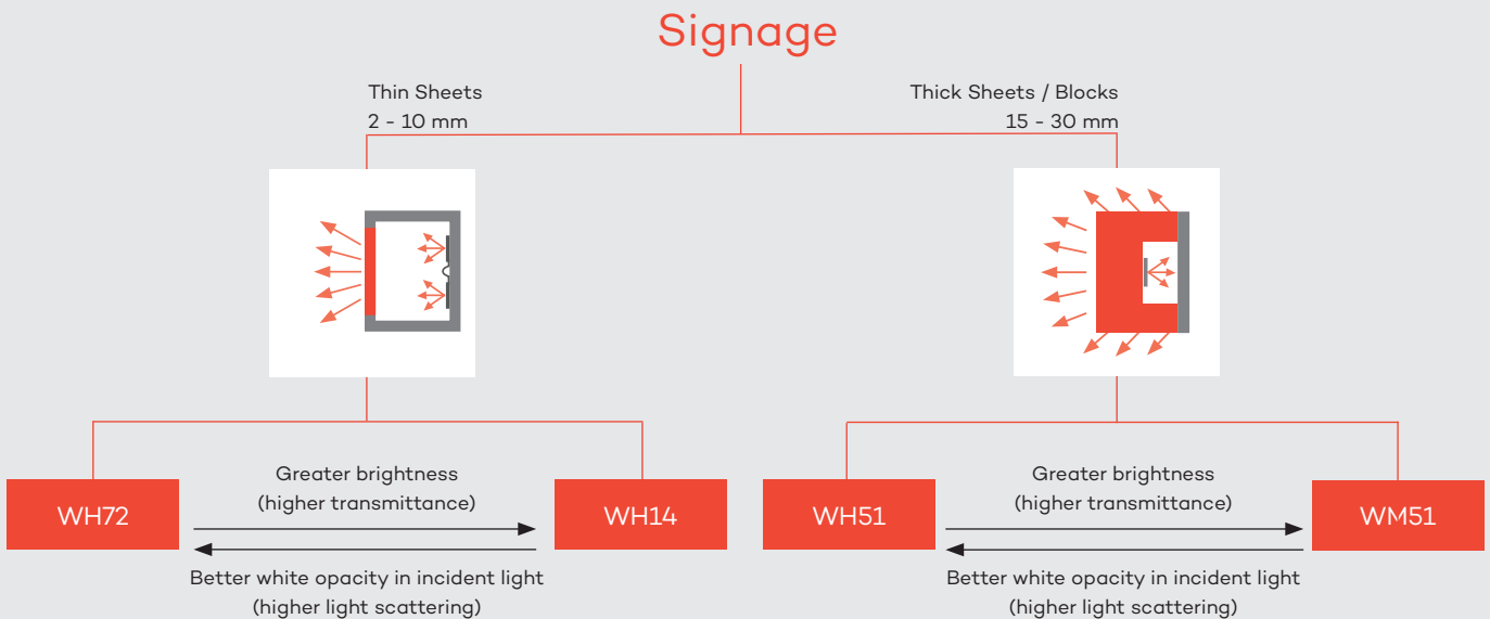
Fig. 3: Decision tree
